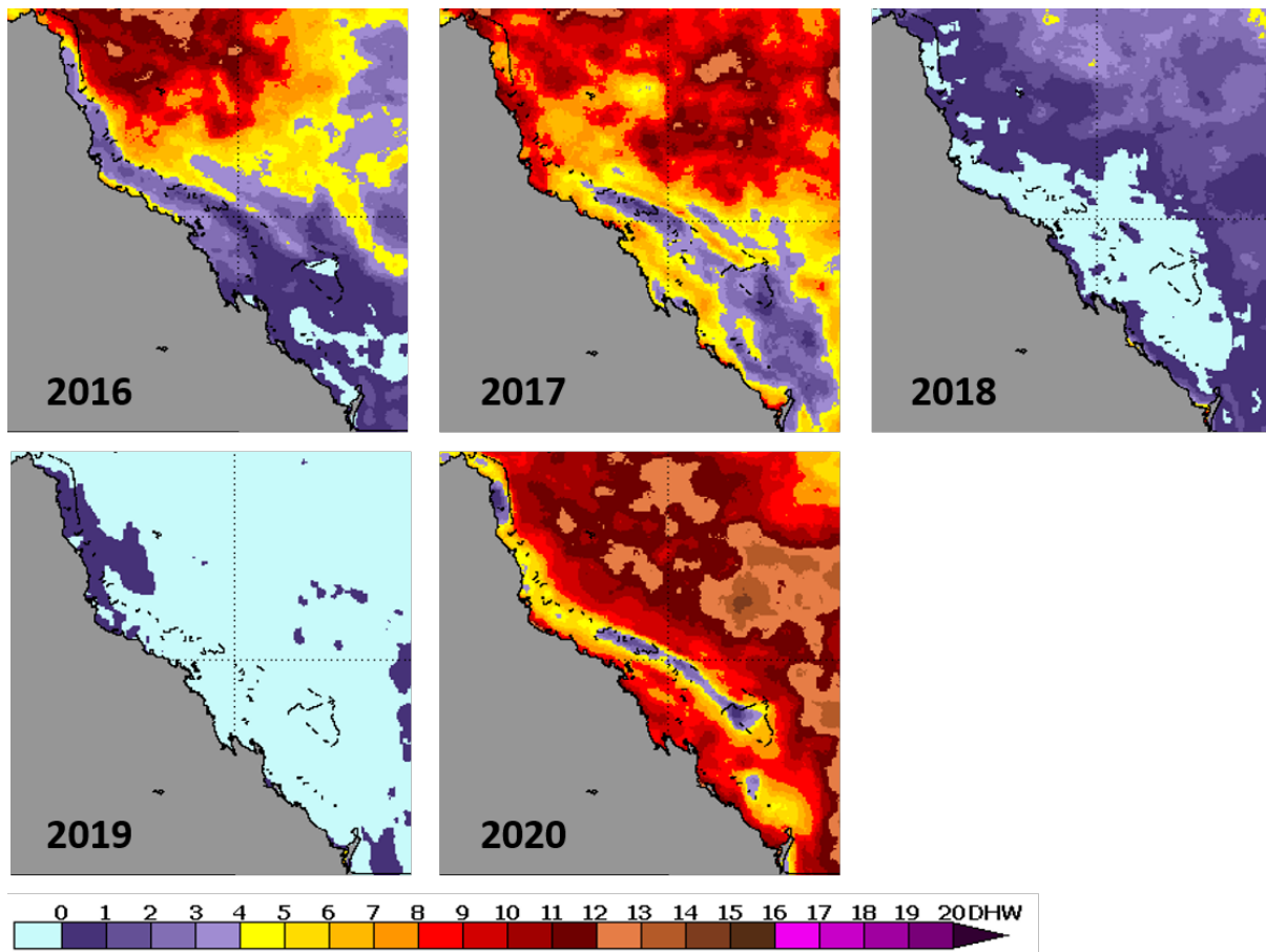
Figure 3 Degree heating week estimates. Images were cropped from regional images sourced from NOAA Coral Reef Watch for the 30th March each Year.
