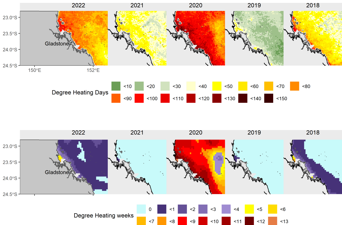
Figure 4 Annual degree heating day and maximum degree heating week estimates. Values of eight are considered the threshold for severe coral bleaching (Lui et al. 2006).
