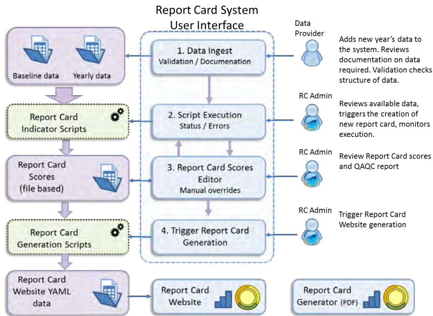
Figure 9.2 | Schematic diagram of the report card system showing all data ingestion, script execution and report cards results generation modules (Diagram courtesy Australian Institute of Marine Science).
