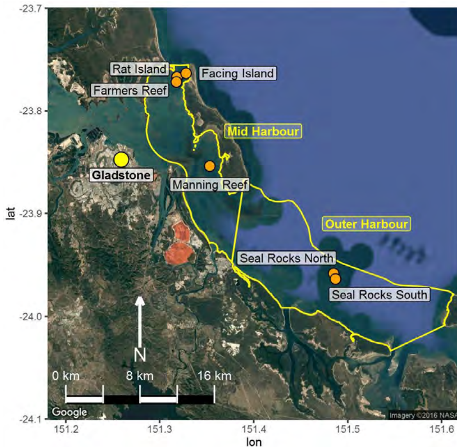
Figure 3.7 | Gladstone Harbour Coral monitoring sites (Thompson et al, 2023).
