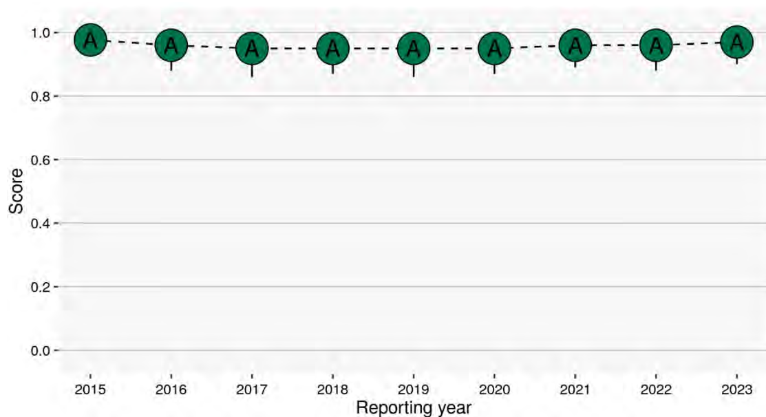
Figure 3.3 | Trends in the overall harbour score for Sediment quality 2015–23 (Error bars show 95% bootstrap confidence intervals).
