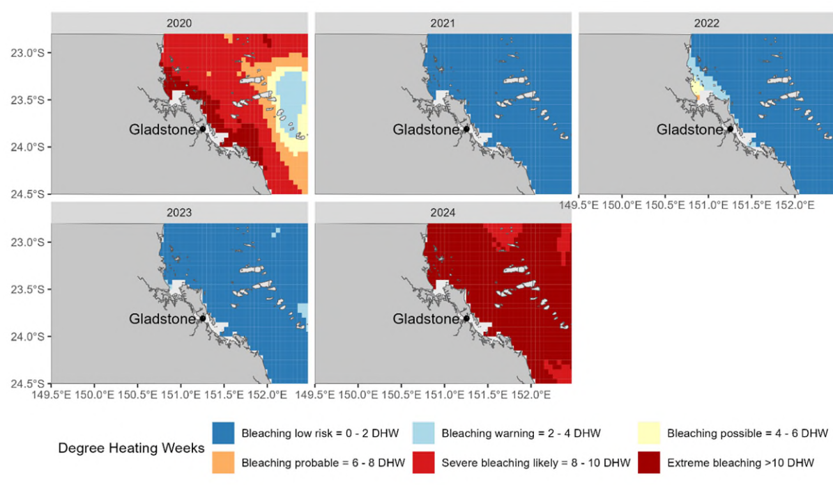
Figure 4 Annual maximum Degree Heating Week estimates.
