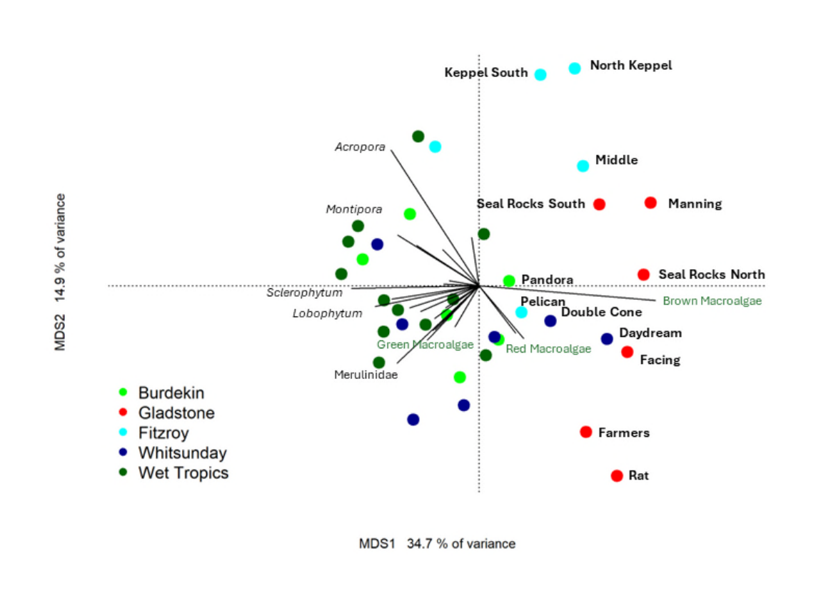
Figure 11 Ordination comparing Gladstone Harbour reef communities with other near-shore reefs. The biplot is based on Bray Curtis dissimilarity of square root transformed cover of coral (genus or family – vectors with black text) and higher order-level cover of macroalgae (vectors with green text) observed on the Gladstone Harbour reefs in 2024 and at 2 m reefs sampled by the Marine Monitoring Program (MMP) in 2023. Labels on the axis indicate how much of the variance in community composition is captured by the first (x-axis, MDS1) and second (y-axis, MDS2) dimensions of the ordination. Reef names are black bolded text
