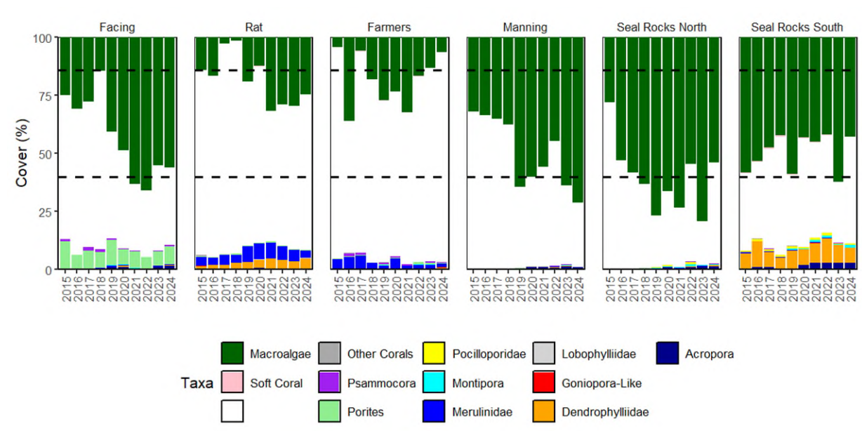
Figure 6 Composition of benthic cover at each location. Rising bars break down coral cover into major taxonomic groups (Families and Genera). Hanging bars represent macroalgae cover and are read in reverse (observed cover is read as 100 – y axis value, i.e. 10% cover will appear as a bar between 100 and 90% on the plot). White space is the remaining cover not occupied by indicators and will include: sand and silt substrate, turfing and crustose coralline algae along with other organisms such as sponges. Dashed reference lines indicate the boundary between the condition categories 'Poor' and 'Satisfactory'. Hanging macroalgae cover bars not extending to the upper dashed reference line would be categorised as 'Satisfactory', or better. Rising bars for coral cover would have to extend to the lower dashed reference line to receive a 'Satisfactory' categorisation.
