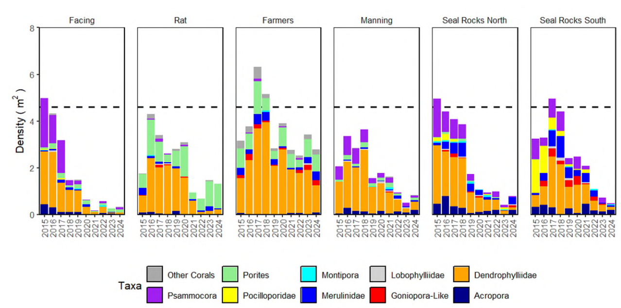
Figure 9 Composition of juvenile coral communities at each location. Bars break down juvenile density into major taxonomic groups (Families and Genera). Dashed reference line indicates the boundary between the condition categories ‘Poor’ and ‘Satisfactory’. Juvenile density would have to extend to the reference line to receive a ‘Satisfactory’ categorisation.
