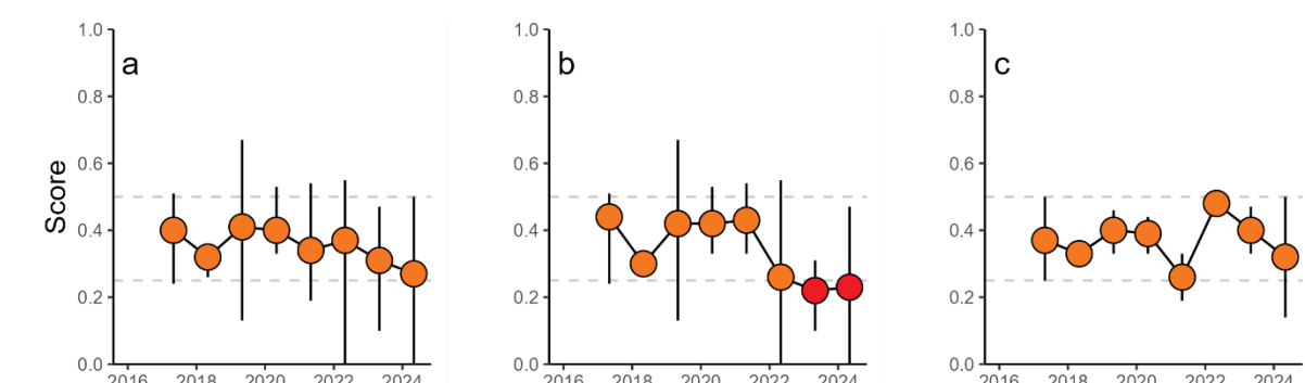
Figure 10 Coral cover change timeseries. Scores for a) Harbour, b) Mid Harbour and c) Outer harbour. Dashed reference lines included for lower thresholds for ‘Satisfactory’ and ‘Poor’ condition categorisations.
