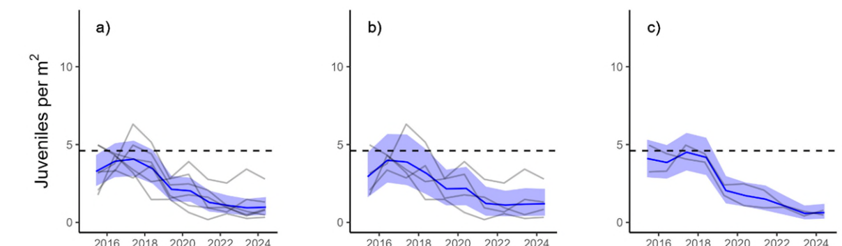
Figure 8 Trends in juvenile density for reporting zones. a) Gladstone Harbour, b) Mid Harbour, c) Outer Harbour. Trends shown by blue lines bound by 95% confidence intervals of those trends (shading), grey lines represent observed profiles for individual reefs. Dashed lines represent the level at which this sub-indicator transitions between ‘poor’ and ‘satisfactory’ report card scores.
