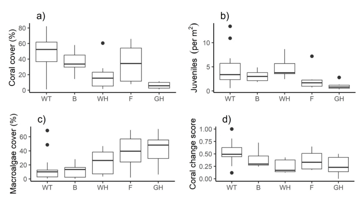
Figure 12 Regional comparisons of sub-indicators. a) coral cover, b) juvenile density, c) macroalgae cover, d) coral change score. WT= Wet Tropics, B=Burdekin, WH=Whitsundays, F= Fitzroy, GH= Gladstone Harbour. Data are based on current indicator values and scores for Gladstone Harbour reefs and the most recent available data for 2 m reefs sampled by the MMP.
